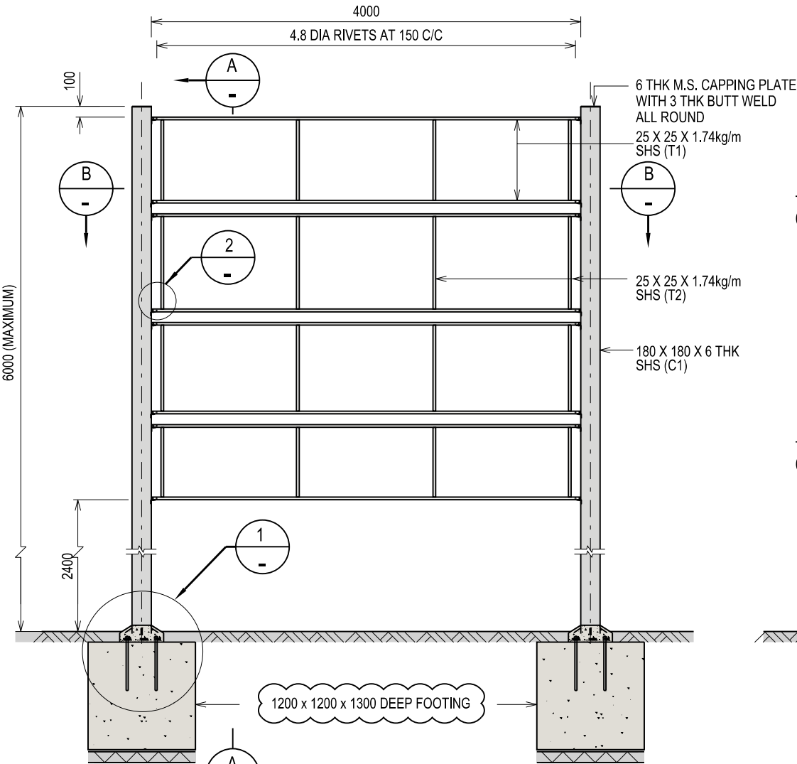
REAR ELEVATION OF PROJECT SIGN BOARD SCALE 1:50
