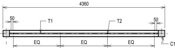
SECTION B-B SCALE 1:50
