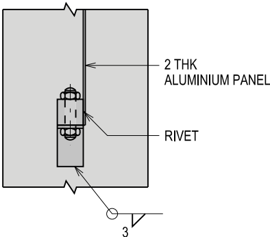
SECTION D-D SCALE 1:5
