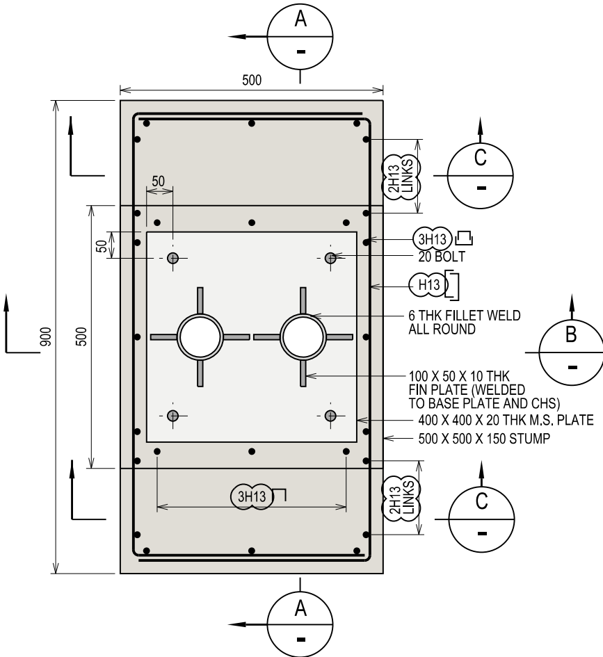
PLAN OF FOUNDATION (FOOTING SIZE = 900mm(L) x 500mm(B) x 500mm(D)) SCALE 1:10
