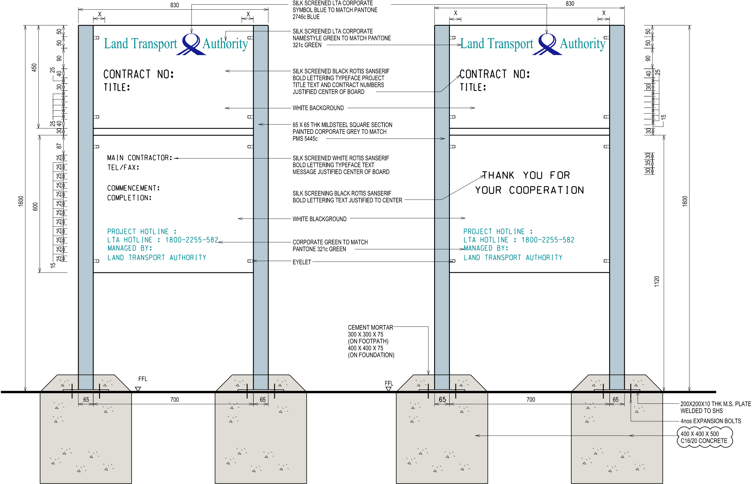
FRONT ELEVATION OF PROJECT SIGNBOARD SCALE 1:10
