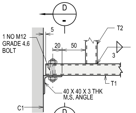
DETAIL 2 SCALE 1:5
