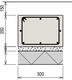
SECTION C-C SCALE 1:20
