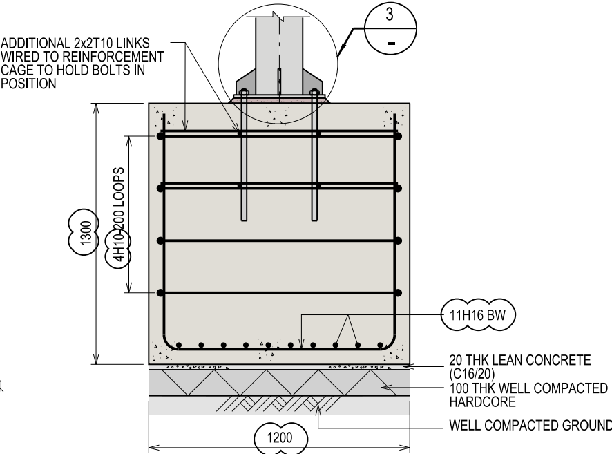
TYPICAL FOOTING DETAILS SCALE 1:20 (CLEAR COVER TO REINFORCEMENT SHALL BE 50mm)
