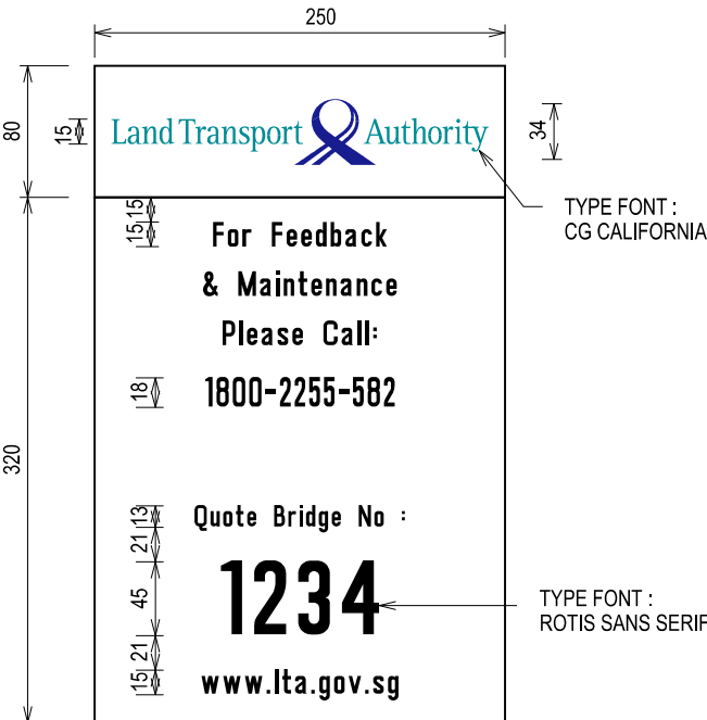
BRIDGE INFORMATION SIGN SCALE 1:5
