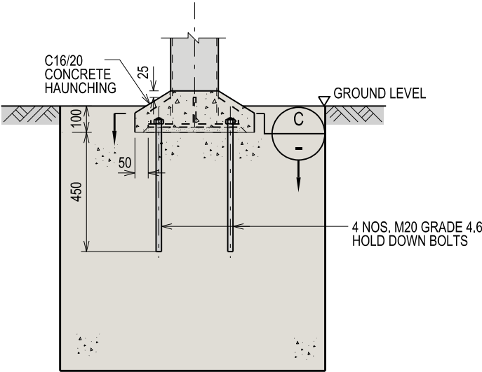
DETAIL 1 TYPICAL BASE PLATE CONNECTION DETAILS SCALE 1:20
