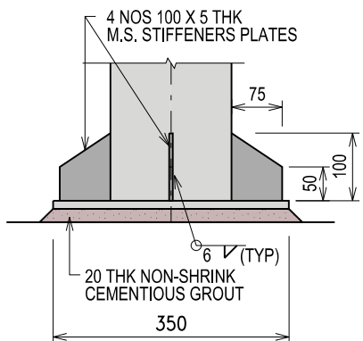
DETAIL 3 5mm THK M.S. STIFFENER DETAILS SCALE 1:10
